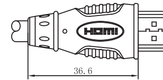
Type A Connector Pin Assignment
