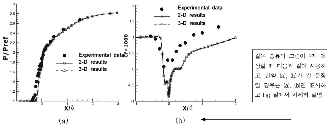
Fig. 2 (a) Wall pressure and (b) skin friction distribution comparison for the 16°compression ramp
